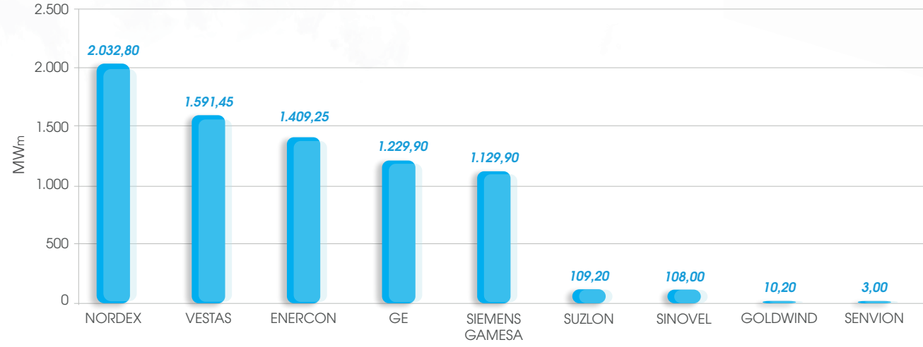
TÜRBİN MARKASI / TURBINE MANUFACTURERS
