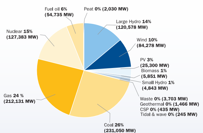
EU POWER CAPACITY MIX 2010
