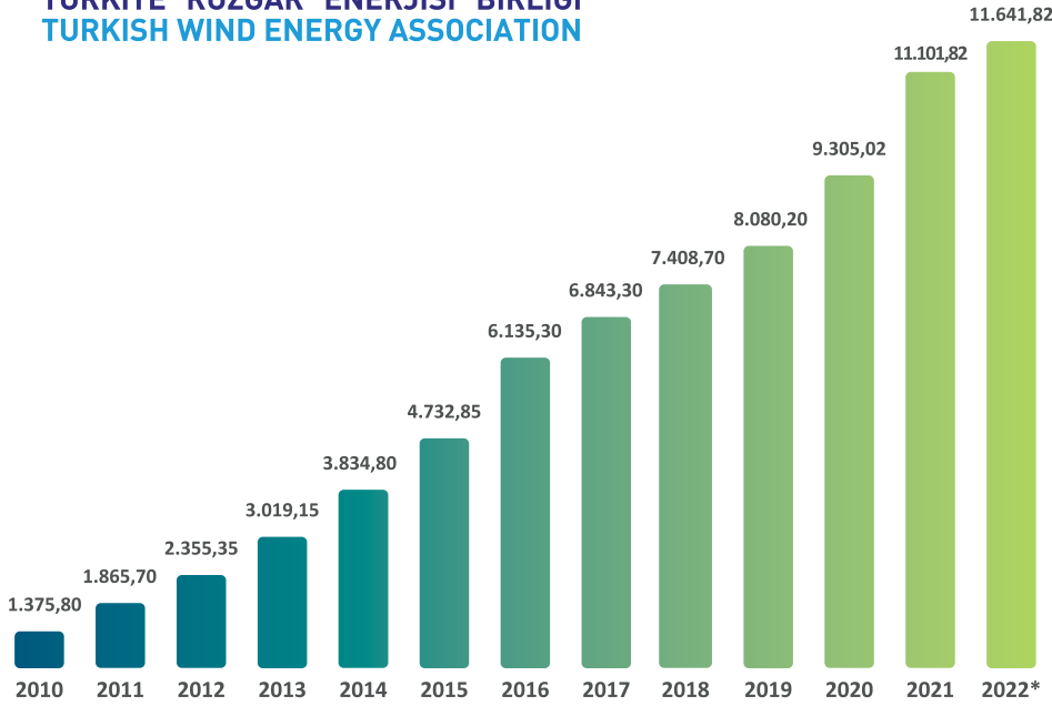
Cumulative Installations for Wind Power Plants in Turkey
